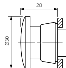
Ø30mm Mushroom button
